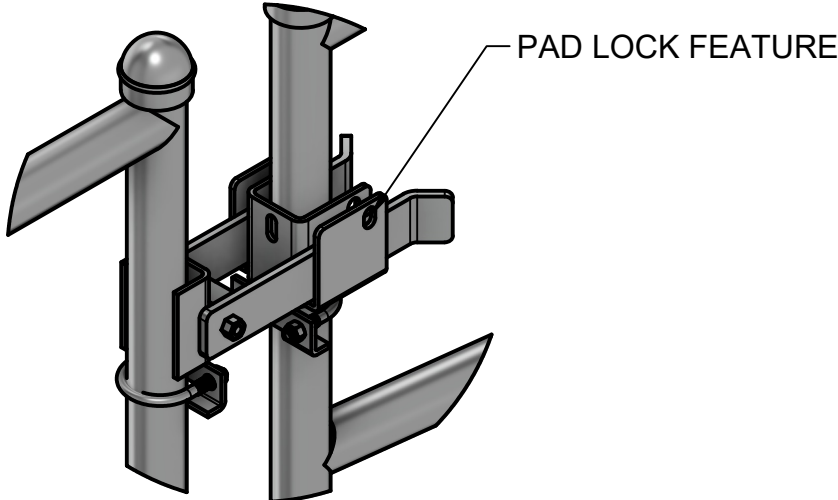
LATCH DETAIL B
